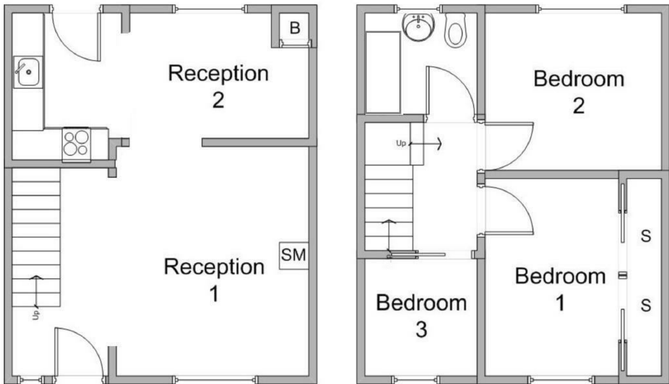
Floor Plan
